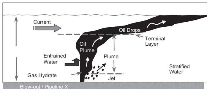
Schematic diagram depicting the basic physical processes involved in a deepwater subsurface oil and gas release.
